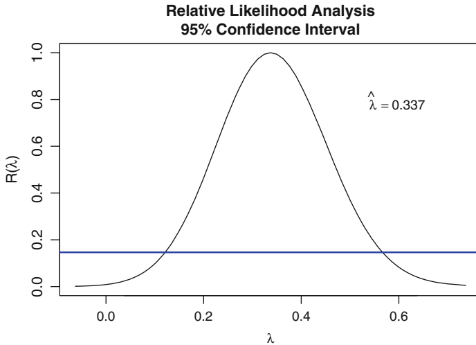
Fig. 13.5. Profile likelihood for \alpha (called \lambda in the legend) in the housing start example. Values of \lambda with R(\lambda) (the profile likelihood) above the horizontal line are in the 95 % confidence limit.
