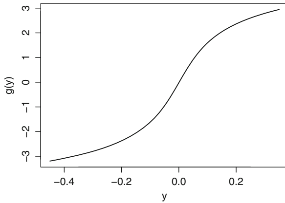
Fig. 5.15. Plot of the transformation used in Example 5.8.
