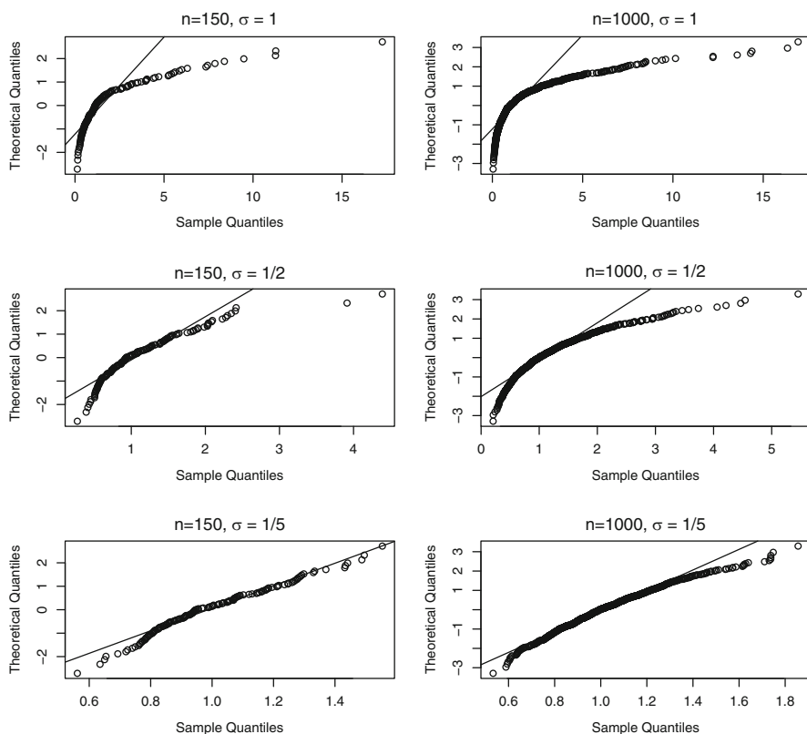
Fig. 4.11. Normal probability plots of random samples of sizes 150 and 1000 from lognormal populations with \mu = 0 and \sigma = 1, 1/2 , or 1/5 . The reference lines pass through the first and third quartiles.
