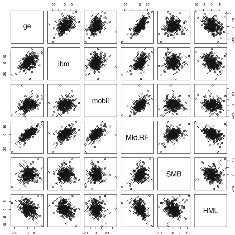
Fig. 18.7. Scatterplot matrix of the excess returns on GE, IBM, and Mobil and the three factors in the Fama–French model. Mkt.RF is the return on the market portfolio minus the risk-free rate.
