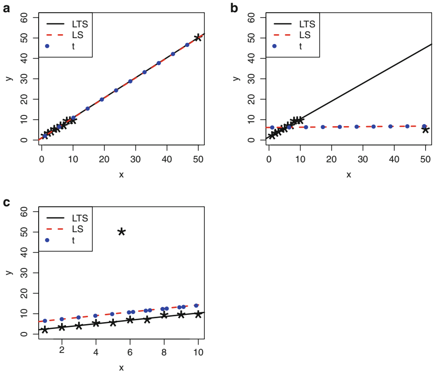
Fig. 11.14. Simulated data in Example 10.1 with LS fits (dashed red) and LTS fits (solid black) and MLEs assuming t -distributed noise (dotted blue). In (a) the three fits are too close together to distinguish between them. In (b) and (c) the LS and t fits are nearly identical and difficult to distinguish.
