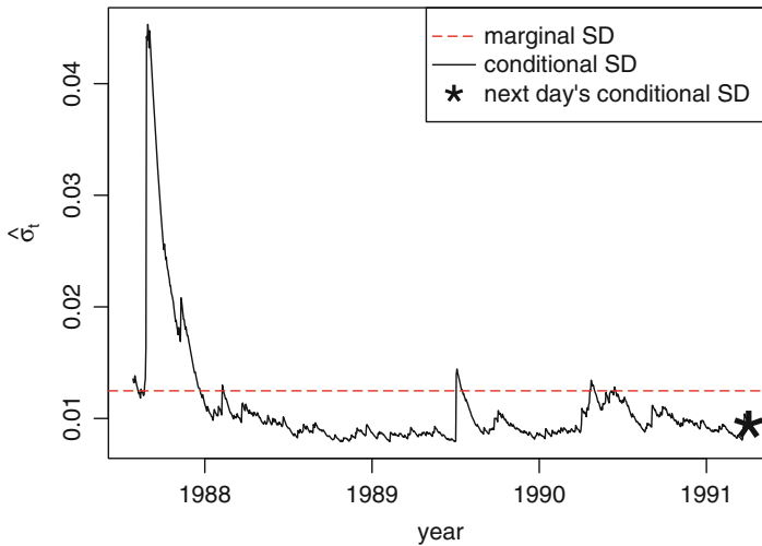
Fig. 19.3. Estimated conditional standard deviation of the daily S&P 500 index returns based on a GARCH(1,1) model. The asterisk is a forecast of the next day's conditional standard deviation from the end of the return series, and the height of the dashed horizontal line is an estimate of the marginal (unconditional) standard deviation.
