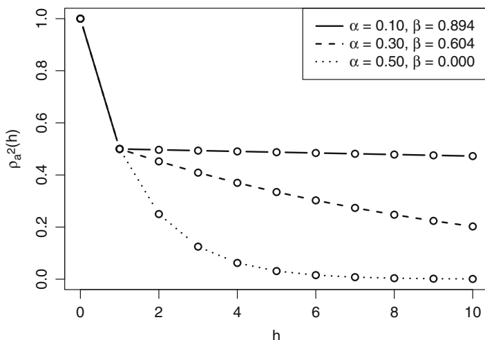
Fig. 14.6. ACFs of three GARCH(1,1) processes with \rho_{a^2}(1) = 0.5 .
