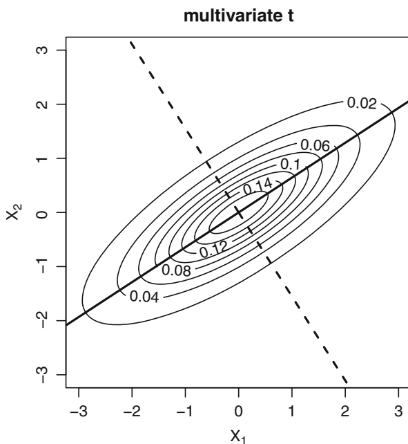
Fig. 7.6. Contour plot of a multivariate t_4 -density with \boldsymbol{\mu} = (0, 0)^\top , \sigma_1^2 = 2 , \sigma_2^2 = 1 , and \sigma_{12} = 1.1 .
