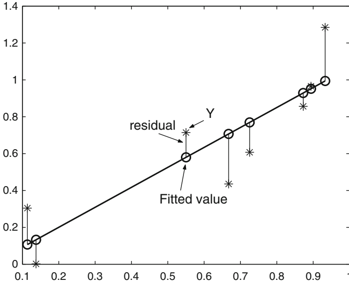
Fig. 9.1. Least-squares estimation. The vertical lines connect the data (*) and the fitted values (o) represent the residuals. The least-squares line is defined as the line making the sum of the squared residuals as small as possible.
