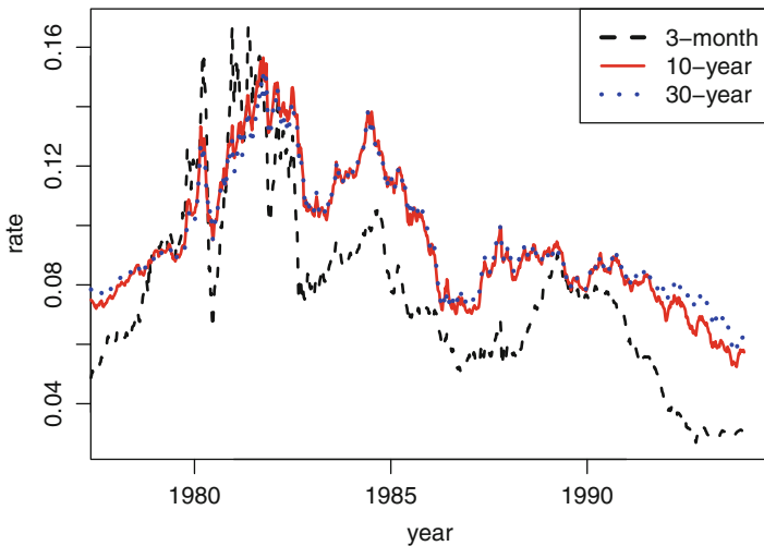
Fig. 3.2. Treasury rates of three maturities. Weekly time series. The data were taken from the website of the Federal Reserve Bank of Chicago.
