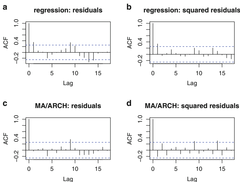
Fig. 14.9. (a) Sample ACF of the externally studentized residuals and (b) their squared values, from a linear model; (c) Sample ACF of the standardized residuals and (d) their squared values, from an MA(1)+ARCH(1) fit to the regression residuals.
