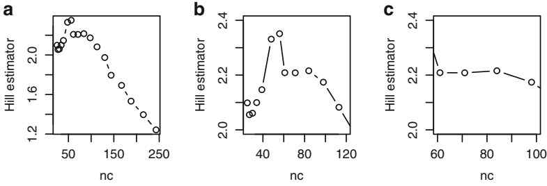
Fig. 19.6. Estimation of the tail index by applying a Hill plot to the daily returns on the S&P 500 index for 1,000 consecutive trading days ending on March 4, 2003. (a) Full range of n_c . (b) Zoom in to n_c between 25 and 120. (c) Zoom in further to n_c between 60 and 100.
