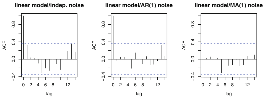
Fig. 13.9. Ice cream consumption example. Residual ACF plots for the linear model with independent noise, the linear model with AR(1) noise, and the linear model with MA(1) noise.
