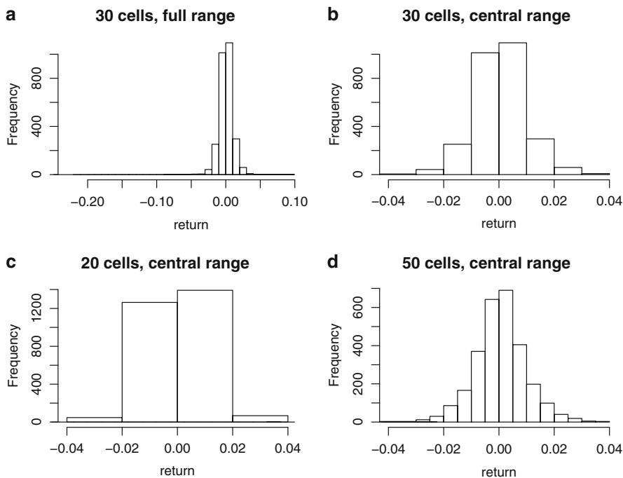
Fig. 4.4. Histograms of the daily log returns on the S&P 500 index from January 1981 to April 1991. This data set is the SP500 series in the Ecdat package in R.
