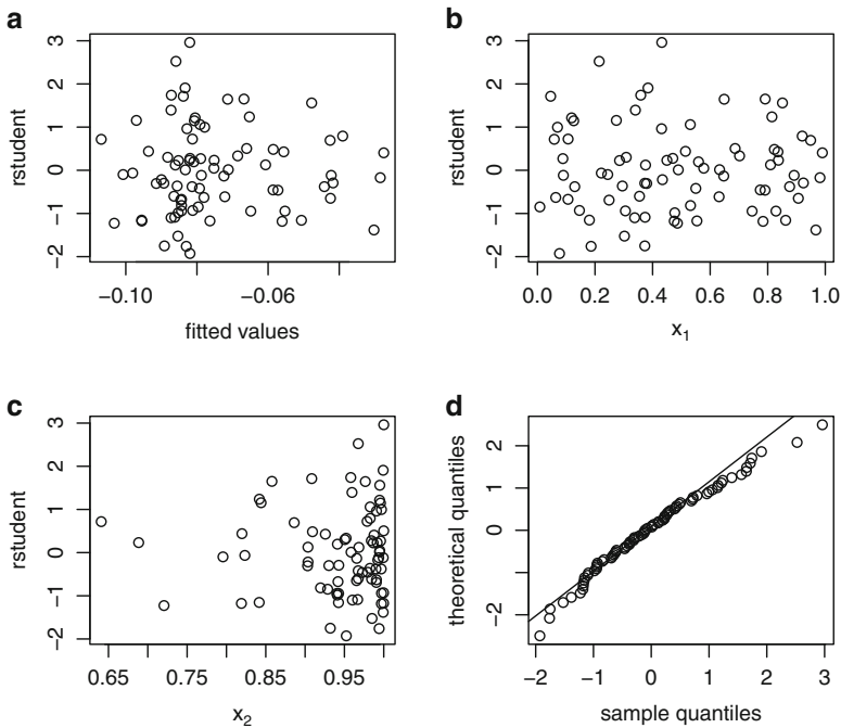
Fig. 11.8. Residuals for the Box-Cox model applied to the simulated data.
