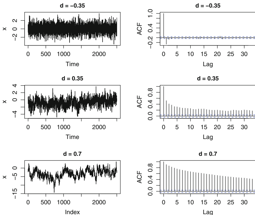
Fig. 13.17. Time series plots (left) and sample ACFs (right) for simulated FARIMA(0, d , 0): the top series is stationary with short-term memory; the middle series is stationary with long-term memory; the bottom series is nonstationary.
