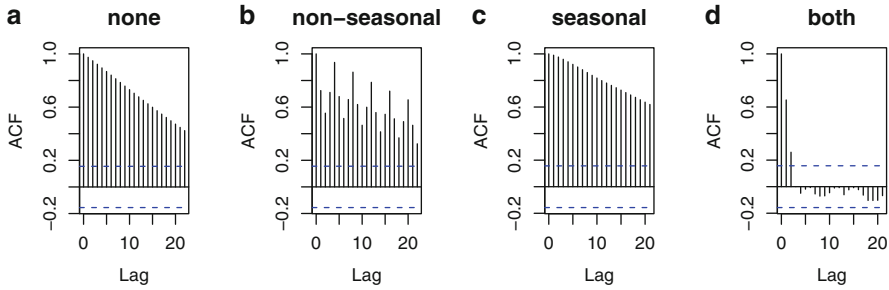
Fig. 13.20. ACF plots of quarterly data with no differencing, nonseasonal differencing, seasonal differencing, and both seasonal and nonseasonal differencing.
