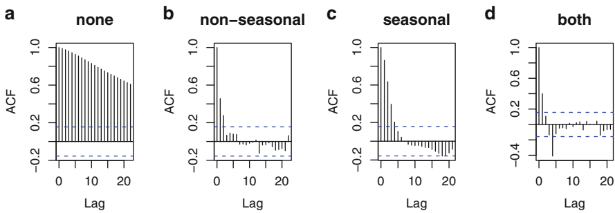
Fig. 13.22. ACF plots of quarterly data with no differencing, nonseasonal differencing, seasonal differencing, and both seasonal and nonseasonal differencing.
