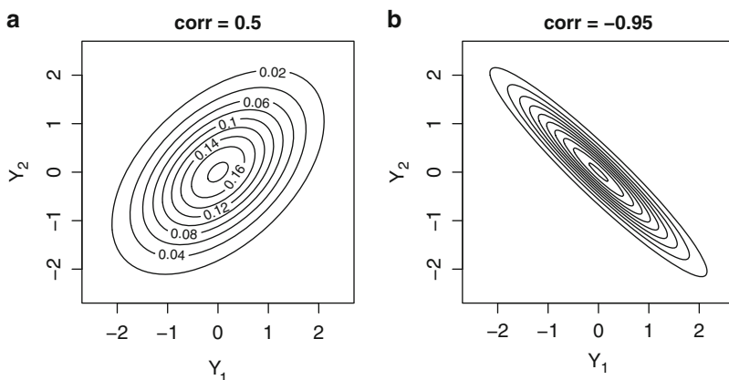
Fig. 7.2. Contour plots of a bivariate normal densities with N(0,1) marginal distributions and correlations of 0.5 or -0.95 .
