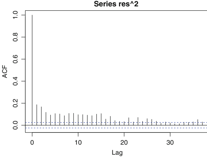
Fig. 14.7. ACF of the squared residuals from an AR(1) fit to the BMW log returns.
