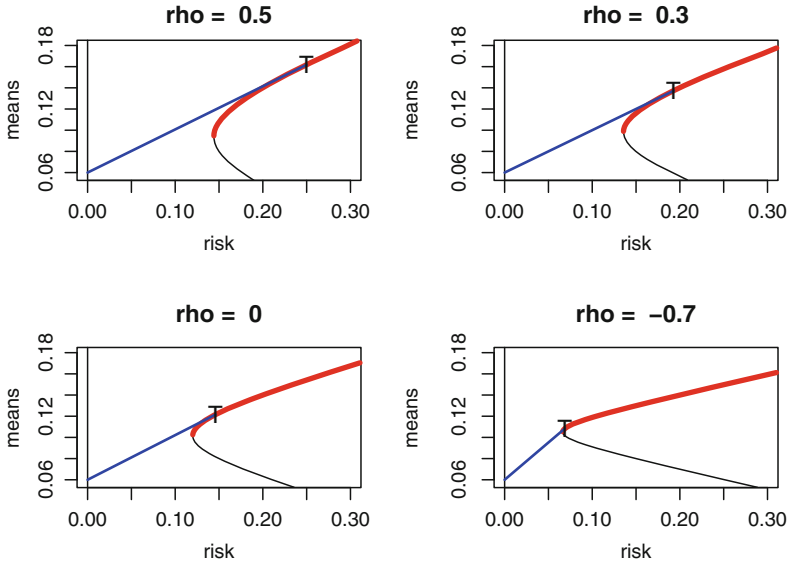
Fig. 16.2. Efficient frontier (red) and tangency portfolio ( T ) when \mu_1 = 0.14 , \mu_2 = 0.09 , \sigma_1 = 0.2 , \sigma_2 = 0.15 , and \mu_f = 0.03 . The value of \rho_{12} is varied from 0.5 to -0.7 .
