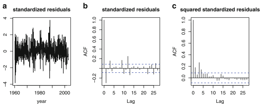
Fig. 21.8. Risk-free monthly returns. Residual analysis. (a) Time series plot of standardized residuals. (b) ACF of standardized residuals. (c) ACF of squared standardized residuals.
