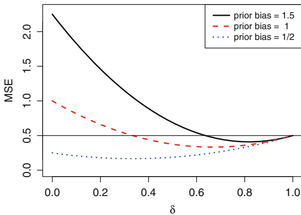
Fig. 20.3. MSE versus \delta for three values of “prior bias” = \mu - \mu_0 when \sigma^2/n = 1/2 . The horizontal line represents the MSE of the maximum likelihood estimator ( \bar{Y} ).
