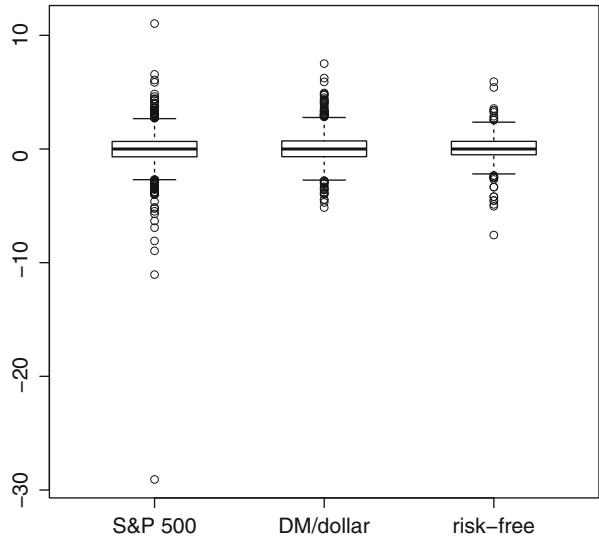
Fig. 4.18. Boxplots of the standardized S&P 500 daily log returns, daily changes in the DM/dollar exchange rate, and monthly changes in the risk-free returns.
