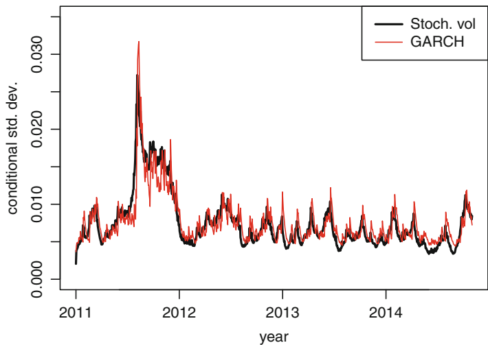
Fig. 20.8. The conditional standard deviations of the log returns estimated by the stochastic volatility model in Example 20.14 and the GARCH(1,1) model.
