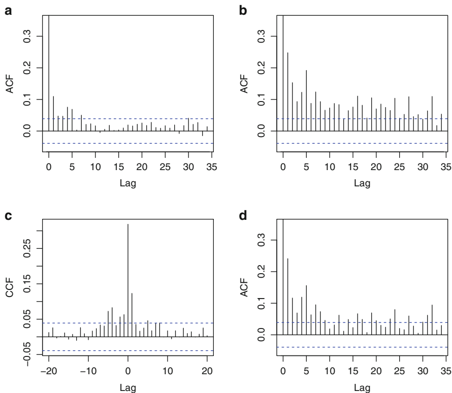
Fig. 14.13. ACFs of squared residuals from a VAR(1) model for (a) IBM and (b) CRSP; (c) CCF between the squared residuals; (d) ACF for the product of the residuals.
