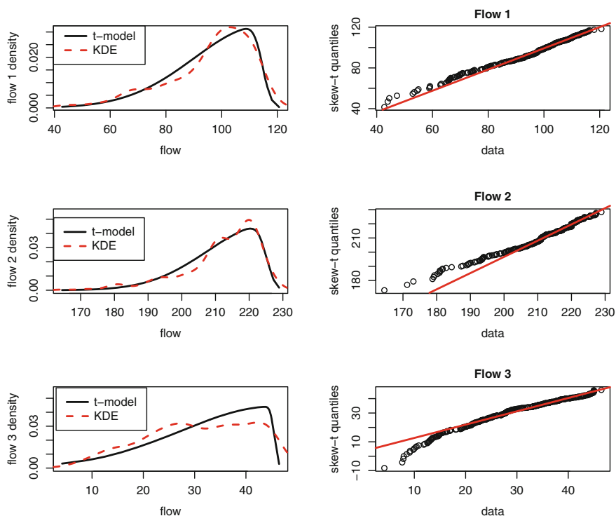
Fig. 5.11. Parametric (solid) and nonparametric (dashed) density estimates for daily flows in three pipelines (left) and QQ plots for the parametric fits (right). The reference lines go through the first and third quartiles.
