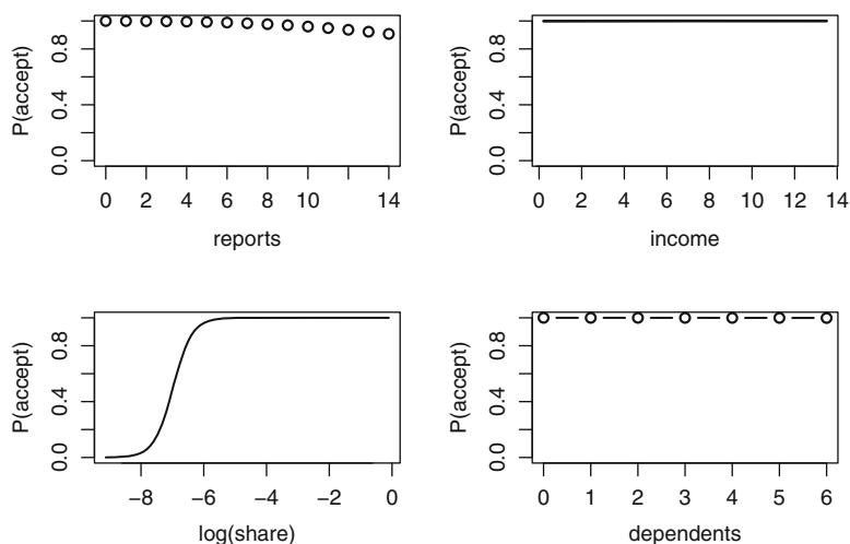
Fig. 11.10. Plots of probabilities of a credit card application being accepted as functions of single predictors with other predictors fixed at their means. The variables vary over their ranges in the data.
