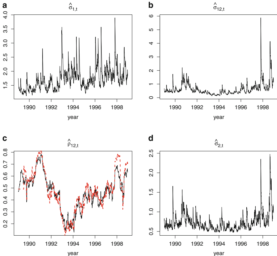
Fig. 14.17. A fitted first order DCC model with (\omega_1, \alpha_1, \beta_1)' = (0.0741, 0.0552, 0.9233)' , (\omega_2, \alpha_2, \beta_2)' = (0.0206, 0.0834, 0.8823)' , and \lambda = 0.9876 . The red line in (c) is the sample correlation estimate over the previous six months for comparison.
