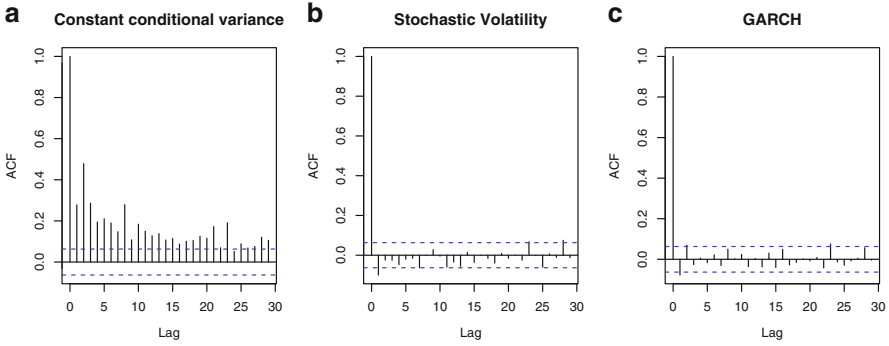
Fig. 20.9. ACF's of the squared standardized residuals. (a) Assuming a constant conditional standard deviation. The model is R_t = \mu + \epsilon_t where \epsilon_t is independent white noise. (b) Assuming an ARMA(1,1) stochastic volatility model. (c) Assuming a GARCH(1,1) model.
