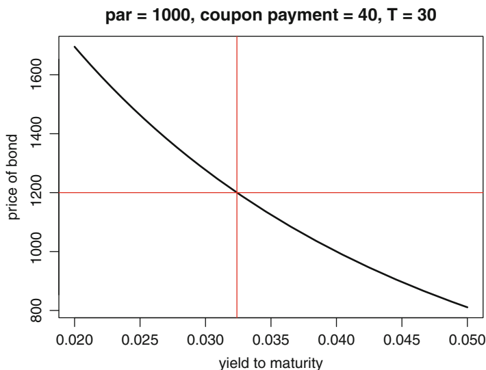
Fig. 3.1. Bond price versus yield to maturity. The horizontal red line is at the bond price of $1,200. The price/yield curve intersects this line at 0.0324 as indicated by the vertical red line. Therefore, 0.0324 is the bond's yield.
