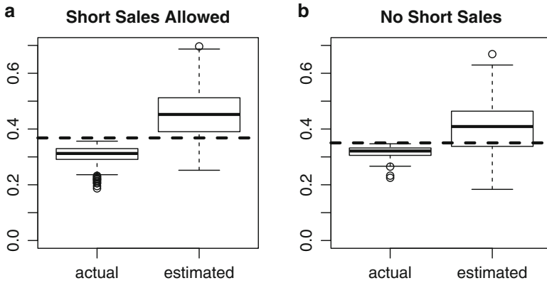
Fig. 16.5. Bootstrapping estimation of the tangency portfolio and its Sharpe's ratio. (a) Short sales allowed. The left-hand boxplot is of the actual Sharpe's ratios of the estimated tangency portfolios for 250 resamples. The right-hand boxplot contains the estimated Sharpe's ratios for these portfolios. The horizontal dashed line indicates Sharpe's ratio of the true tangency portfolio. (b) Same as (a) but with short sales not allowed.
