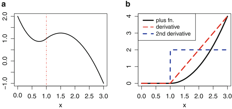
Fig. 21.6. (a) Quadratic spline with a knot at 1. The dotted red vertical line marks the knot's location. (b) The quadratic plus function (x-1)_+^2 with a knot at 1 (black) and its first (red) and second (blue) derivatives.
