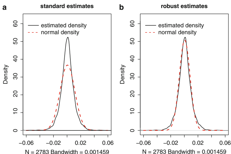
Fig. 4.7. Kernel density estimates (solid) of the daily log returns on the S&P 500 index compared with normal densities (dashed). (a) The normal density uses the sample mean and standard deviation. (b) The normal density uses the sample median and MAD estimate of standard deviation. This data set is the SP500 series in the Ecdat package in R.
