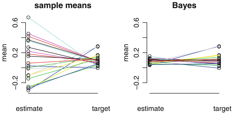
Fig. 20.7. Estimation of the average returns for 20 midcap stocks. “Target” is the quantity being estimated, specifically the average return over 400 days of test data. “Estimate” is an estimate based on the 100 previous days of training data. On the left, the estimates are the 20 individual sample means. On the right, the estimates are the sample means shrunk toward their mean. In each panel, the estimate and target for each stock are connected by a line. On the left, the sample means of the training data are so variable that the stocks with smaller (larger) means in the training data often have larger (smaller) means in the test data. The Bayes estimates on the right are much closer to the targets.
