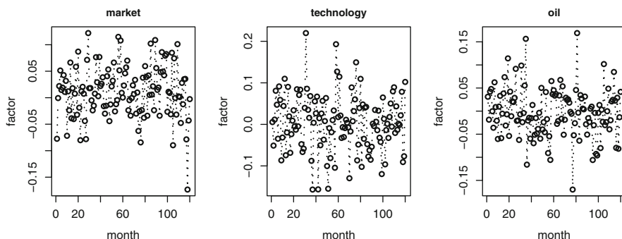
Fig. 18.9. Time series plots of the estimated values of the three factors in the cross-sectional factor model.
