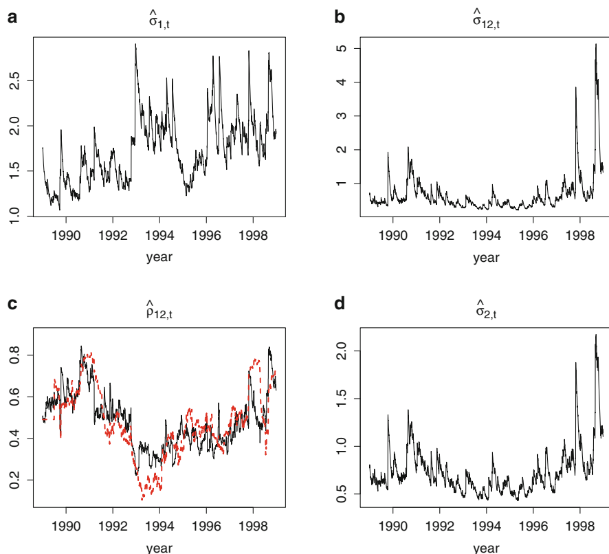
Fig. 14.16. A fitted first order DOCs in volatility GARCH model with (\omega_1, \alpha_1, \beta_1, \nu_1)' = (0.0049, 0.0256, 0.9703, 4.3131)' , (\omega_2, \alpha_2, \beta_2, \nu_2)' = (0.0091, 0.0475, 0.9446, 5.0297)' , and M = ((1.5350, 0.838)', (0.0103, 0.7730)') . The red line in (c) is the sample correlation estimate over the previous six months for comparison.
