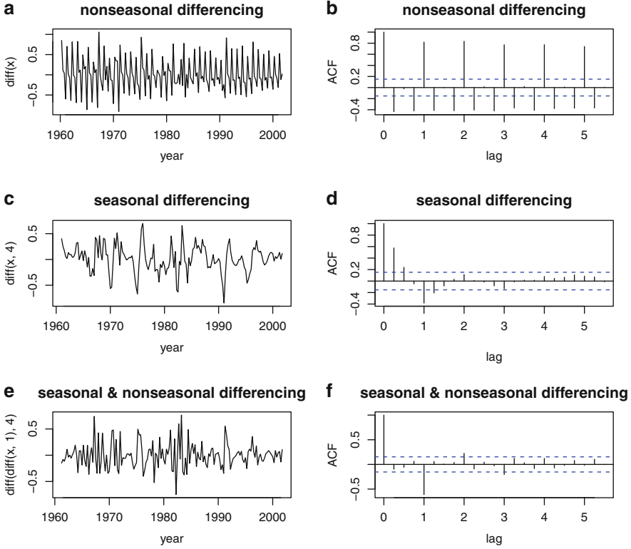
Fig. 13.2. Time series (left column) and sample ACF plots (right column) of the logarithms of quarterly urban housing starts with nonseasonal differencing (top row), seasonal differencing (middle row), and both seasonal and nonseasonal differencing (bottom row). Note: in the sample ACF plots, lag = 1 means a lag of one year, which is four observations for quarterly data.
