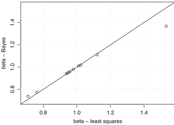
Fig. 20.11. Plot of the Bayes estimator of \beta versus the least-squares estimator.
