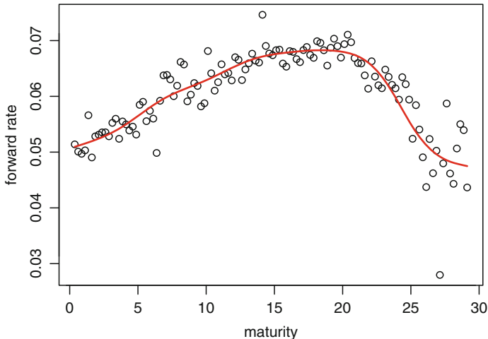
Fig. 21.9. Empirical forward rates (circle) with a spline fit.
