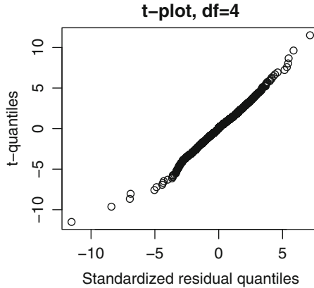
Fig. 14.5. A t -plot with 4 df for the standardized residuals \hat{\epsilon}_t from an AR(1)+GARCH(1,1) model fit to daily BMW stock log return; the reference lines go through the first and third quartiles.
