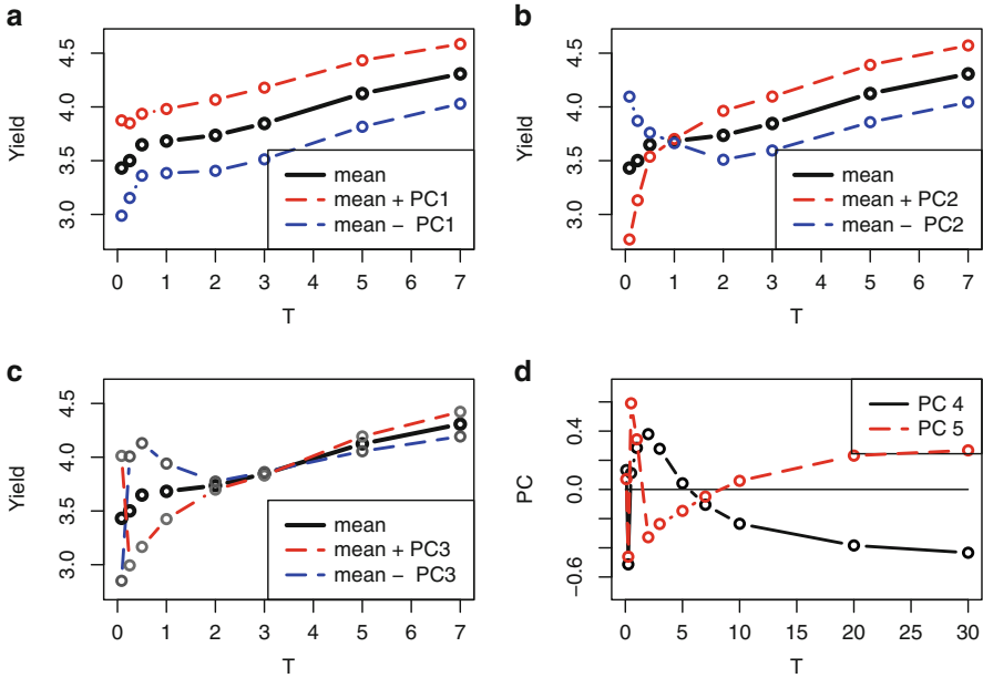
Fig. 18.2. (a) The mean yield curve plus and minus the first eigenvector. (b) The mean yield curve plus and minus the second eigenvector. (c) The mean yield curve plus and minus the third eigenvector. (d) The fourth and fifth eigenvectors for changes in the Treasury yields.
