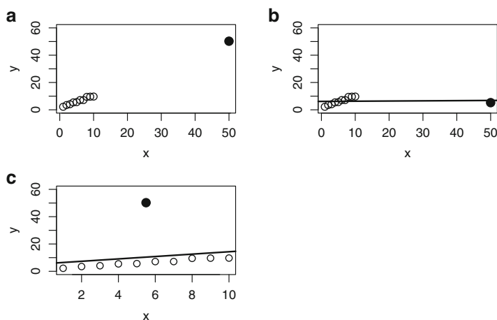
Fig. 10.1. (a) Linear regression with a high-leverage point that is not a residual outlier (solid circle). (b) Linear regression with a high-leverage point that is a residual outlier (solid circle). (c) Linear regression with a low-leverage point that is a residual outlier (solid circle). Least-squares fits are shown as solid lines.
