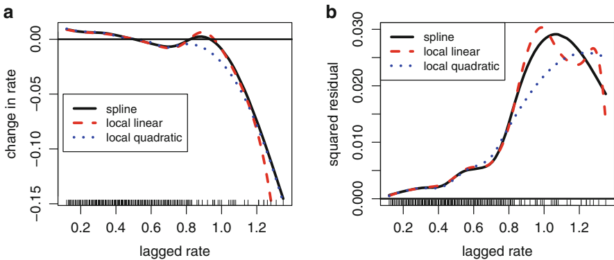
Fig. 21.7. Risk-free monthly returns. (a) Estimates of the drift function. (b) Estimates of the squared volatility function.
