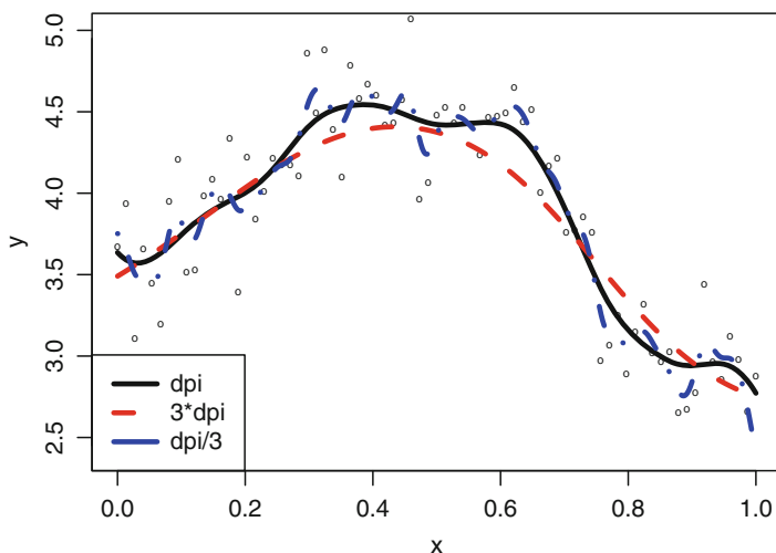
Fig. 21.3. Local linear estimators with three bandwidths: dpi (direct plug-in), which gives an appropriate amount of smoothing; three times the dpi , which oversmooths (underfits); and one-third the dpi , which undersmooths (overfits). Simulated data.
