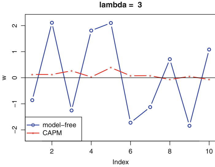
Fig. 20.10. Allocation (or weight) vectors using the sample mean vector and covariance matrix (model-free) and CAPM-based estimates.
