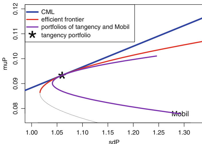
Fig. 17.3. Derivation of the SML. The purple curve is the locus of portfolios combining Mobil stock and the tangency portfolio (asterisk). The purple curve is to the right of the efficient frontier (red) and intersects the efficient frontier at the tangency portfolio. Therefore, the derivative of the purple curve at the tangency portfolio is equal to the slope of the CML (blue), since the purple curve is tangent to the CML at the tangency portfolio.
