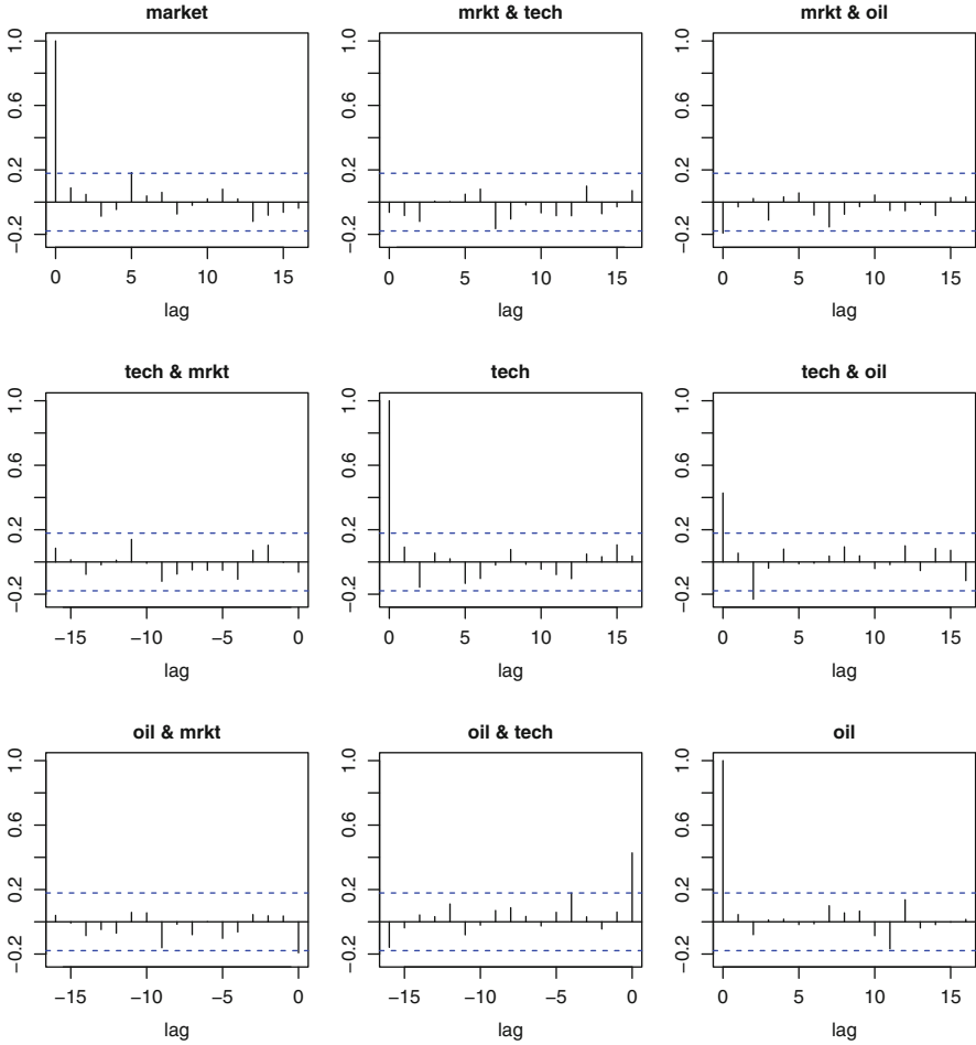
Fig. 18.10. Auto- and cross-correlation plots of the estimated three factors in the cross-sectional factor model. Series 1–3 are the market, tech, and oil factors, respectively.
