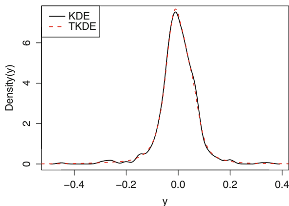
Fig. 5.13. Kernel density and transformation kernel density estimates of monthly changes in the risk-free returns, January 1960 to December 2002. The data are in the Capm series in the Ecdat package in R.
