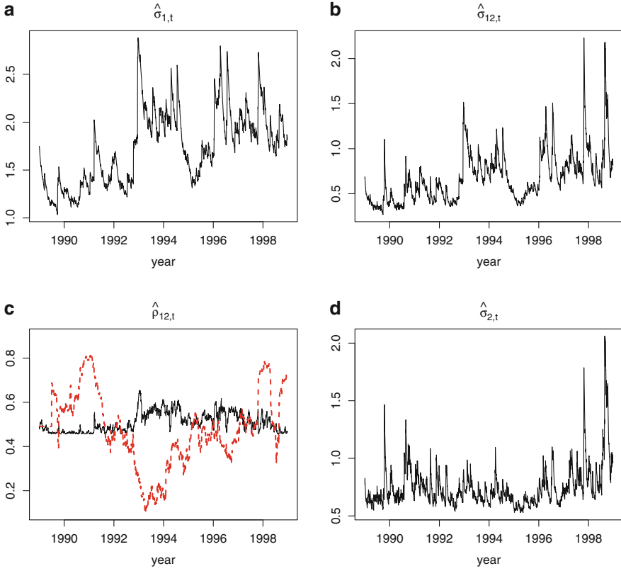
Fig. 14.15. A fitted first order orthogonal GARCH model with (\omega_1, \alpha_1, \beta_1)' = (0.0038, 0.0212, 0.9758)' , (\omega_2, \alpha_2, \beta_2)' = (0.0375, 0.0711, 0.8913)' , and U^{-1} = ((1.7278, 0.2706)', (0.2706, 0.7241)') . The red line in (c) is the sample correlation estimate over the previous six months for comparison.
