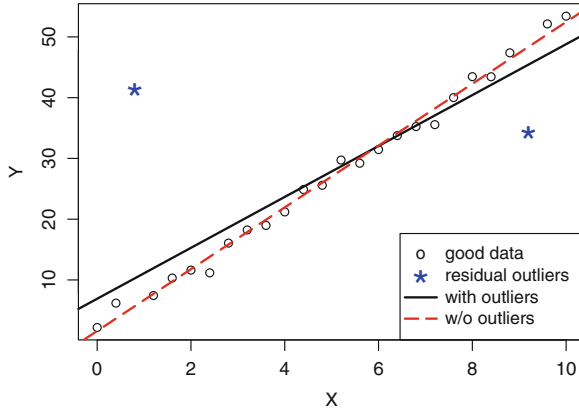
Fig. 11.13. Straight-line regression with two residual outliers showing least-squares fits with and without the outliers.
