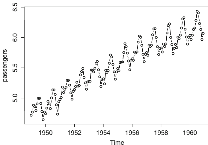
Fig. 13.4. Time series plot of the logarithms of the monthly total international airline passengers (in thousands).
