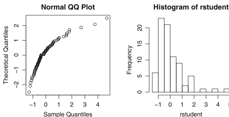
Fig. 10.7. Simulated data. Normal plot and histogram of the studentized residuals. Right skewness is evident and perhaps a square root or log transformation of Y would be helpful.
