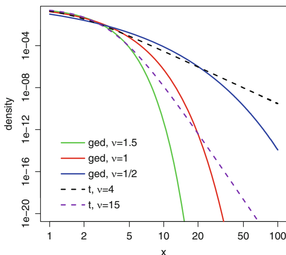
Fig. 5.6. A comparison of the tails of several generalized error (solid curves) and t -distributions (dashed curves).
