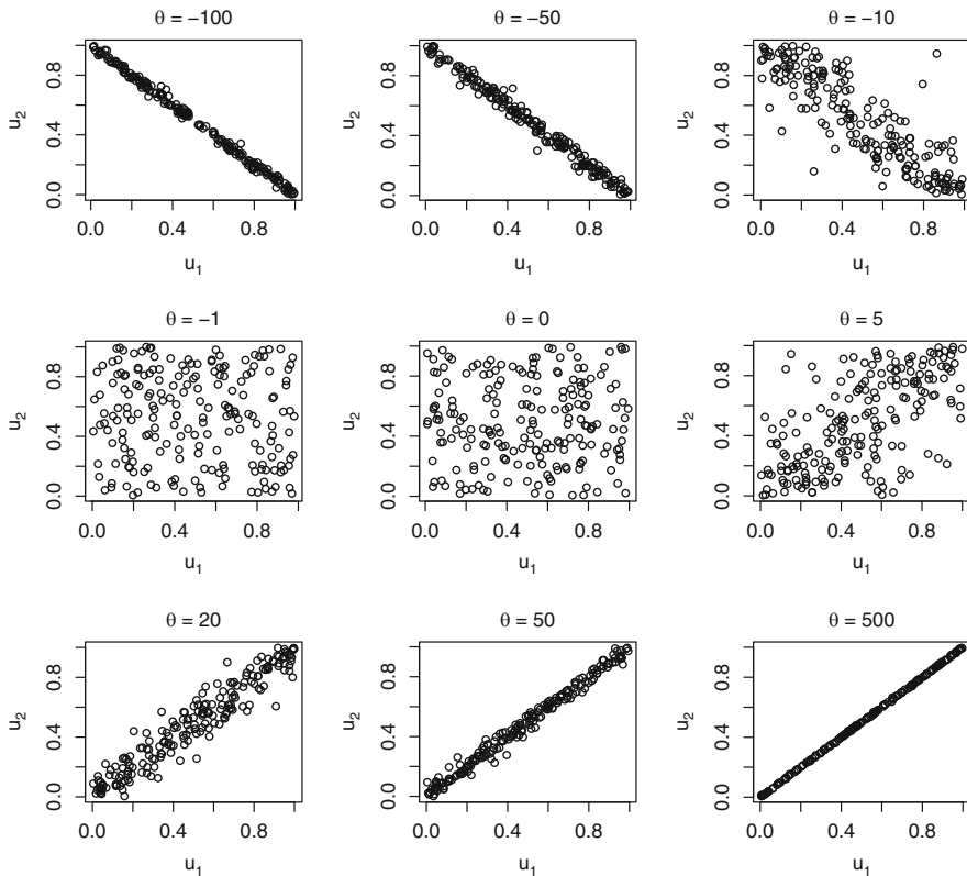
Fig. 8.2. Bivariate random samples of size 200 from various Frank copulas.
