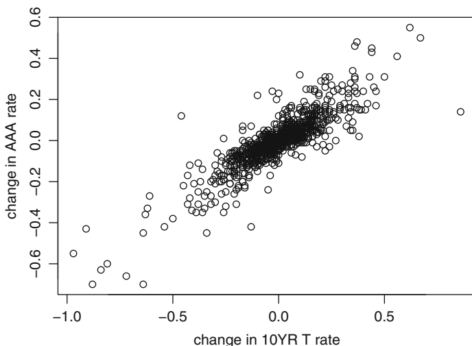
Fig. 9.2. Changes in Moody's seasoned corporate AAA bond yields plotted against changes in 10-year Treasury constant maturity rate. Data from Federal Reserve Statistical Release H.15 and were taken from the Chicago Federal Bank's website.
