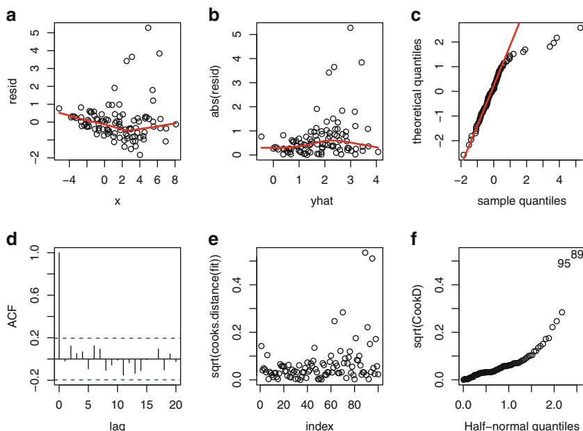
Fig. 10.13. Residual plots and diagnostics for regression of Y on X in Problem 4. The residuals are rstudent values. (a) Plot of residual versus x . (b) Plot of absolute residuals versus fitted values. (c) Normal Q-Q plot of residuals. (d) ACF plot of residuals. (e) Plot of the square root of Cook's D versus index (= observation number). (f) Half-normal plot of square root of Cook's D .
