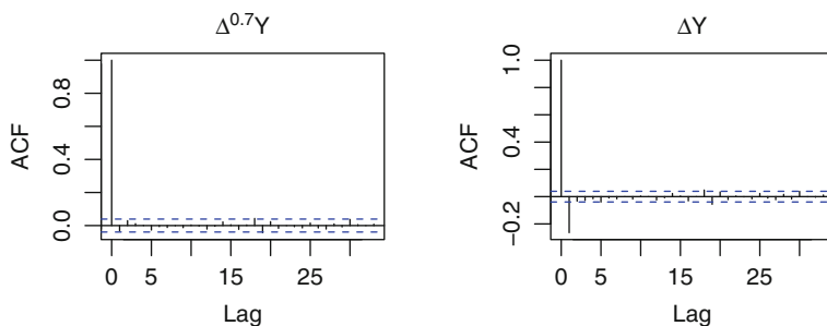
Fig. 13.18. Sample ACF plots for the simulated FARIMA(0, 0.7, 0) series in Figure 13.17 after differencing using d = 0.7 and 1.
