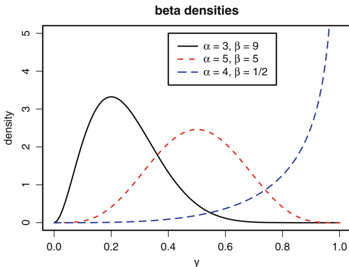
Fig. A.3. Examples of beta probability densities with differing shape parameters.
