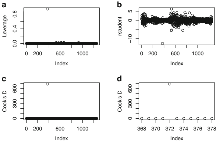
Fig. 10.5. Weekly interest data. Regression of aaa_dif on cm10_dif and cm30_dif . Full data set including the first 371 weeks of data where cm30 was missing and assigned a value of 0. This caused severe problems at case number 372, which are detected by the leverages in (a), rstudent in (b), and Cook's D in (c). Panel (d) zooms in on the outlier case to identify the case number as 372.
