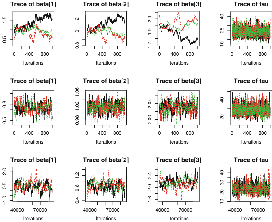
Fig. 20.5. MCMC analysis of a linear regression model with two predictor variables. Simulated data. Trace plots of the regression coefficients and residual precision for three chains. The burn-in period was 100 and the chain lengths are 1000. The trace plots contain the MCMC output after the burn-in period. The intercept is beta[1] and the slopes are beta[2] and beta[3]. Top row: The two predictors are highly correlated and the strong collinearity is causing poor mixing of the regression coefficients. Notice that the chains have not converged to the stationary distribution by the start of the sampling period and that the between-chain variation is large. Middle row: The burn-in period was 100 and the chain lengths are 1000 as in the top row. The two predictors are independent and there is very good mixing because there is no collinearity. Notice that the chains have converged to the stationary distribution by the start of the sampling period and there is little between-chain variation. Bottom row: Same data set as the top row but with a burn-in period of 5000 and chain lengths of 30,000. The chains have been thinned so that only every 10th iteration is retained.
