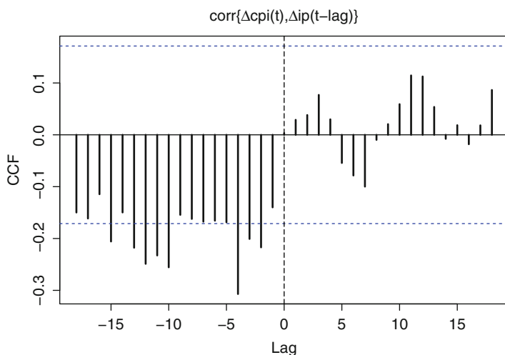
Fig. 13.12. Sample CCF for \Delta cpi and \Delta ip . Note the negative correlation at negative lags, that is, between the cpi and future values of ip .
