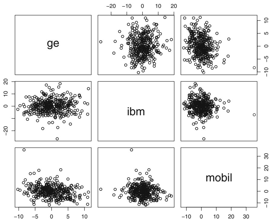
Fig. 18.8. Scatterplot matrix of the residuals for GE, IBM, and Mobil from the Fama–French model.
