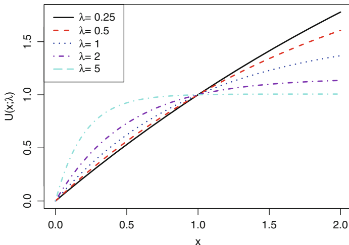
Fig. 16.7. The utility functions \tilde{U}(x; \lambda) = U(x; \lambda)/U(0, \lambda) where U(x; \lambda) = 1 - \exp(-\lambda x) .
