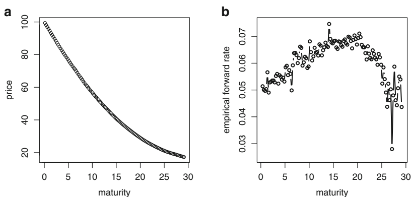
Fig. 11.4. (a) U.S. STRIPS prices. (b) Empirical forward-rate estimates from the prices.
