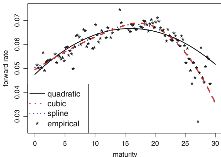
Fig. 11.5. Polynomial and spline estimates of forward rates of U.S. Treasury bonds. The empirical forward rates are also shown.
