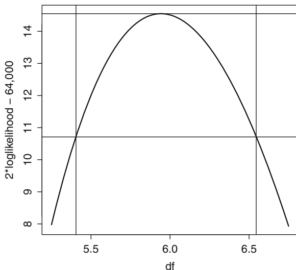
Fig. 7.5. CRSPday data. A profile likelihood confidence interval for \nu . The solid curve is 2L_{\max}(\nu) , where L_{\max}(\nu) is the profile likelihood minus 32,000. 32,000 was subtracted from the profile likelihood to simplify the labeling of the y-axis. The horizontal line intersects the y-axis at 2L_{\max}(\hat{\nu}) - \chi^2_{\alpha,1} , where \hat{\nu} is the MLE and \alpha = 0.05 . All values of \nu such that 2L_{\max}(\nu) is above the horizontal line are in the profile likelihood 95 % confidence interval. The two vertical lines intersect the x-axis at 5.41 and 6.55, the endpoints of the confidence interval.
