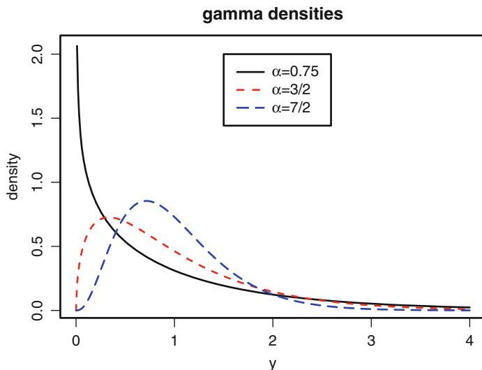
Fig. A.2. Examples of gamma probability densities with differing shape parameters. In each case, the scale parameter has been chosen so that the expectation is 1.
