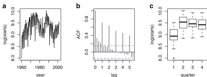
Fig. 13.1. Logarithms of quarterly urban housing starts in Canada: (a) time series plot; (b) sample ACF; (c) boxplots by quarter.
