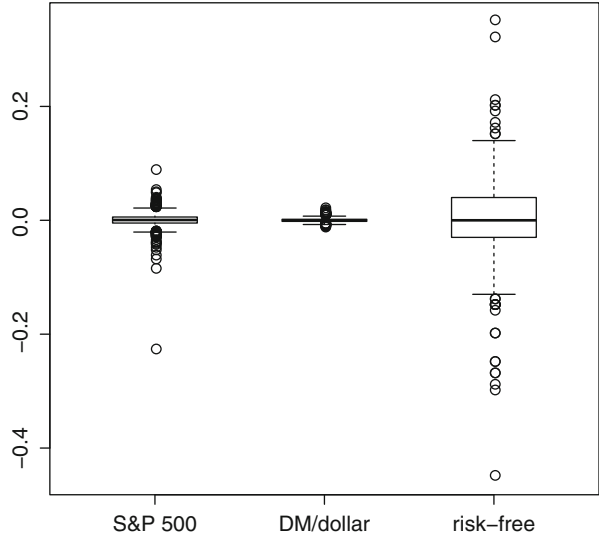
Fig. 4.17. Boxplots of the S&P 500 daily log returns, daily changes in the DM/dollar exchange rate, and monthly changes in the risk-free returns.
