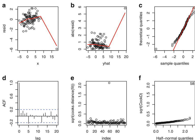
Fig. 10.11. Residual plots and diagnostics for regression of Y on X in Problem 2. The residuals are rstudent values. (a) Plot of residual versus x . (b) Plot of absolute residuals versus fitted values. (c) Normal Q-Q plot of residuals. (d) ACF plot of residuals. (e) Plot of the square root of Cook's D versus index (= observation number). (f) Half-normal plot of square root of Cook's D .
