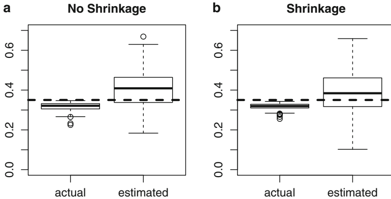
Fig. 16.6. Bootstrapping estimation of the tangency portfolio and its Sharpe's ratio. Short sales not allowed. (a) No shrinkage. The left-hand boxplot is of the actual Sharpe's ratios of the estimated tangency portfolios for 250 resamples. The right-hand boxplot contains the estimated Sharpe's ratios for these portfolios. The horizontal dashed line indicates Sharpe's ratio of the true tangency portfolio. (b) Same as (a) but with shrinkage.
