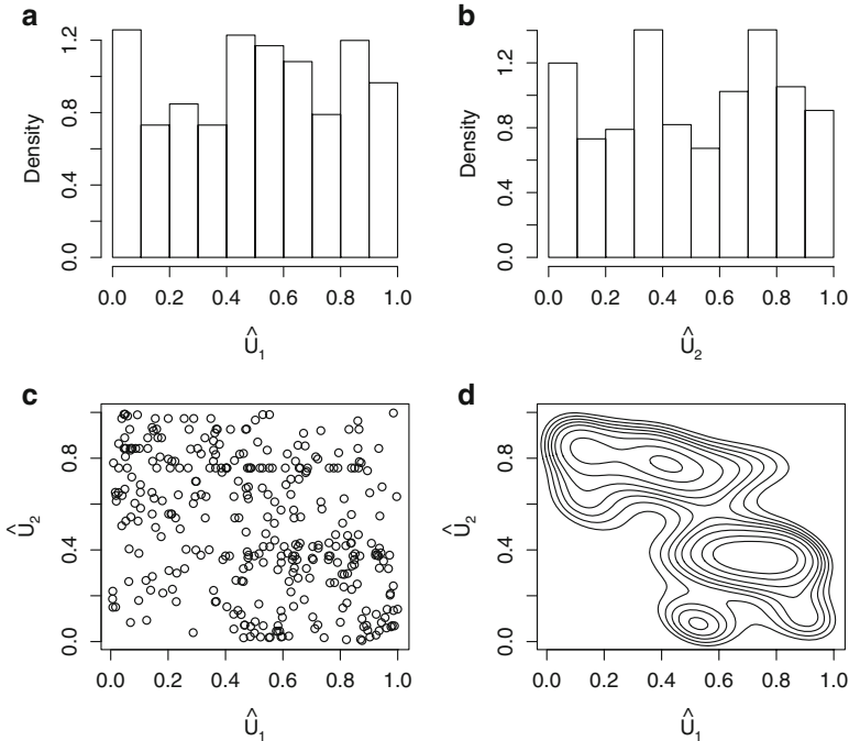
Fig. 8.7. Pipeline data. Density histograms (a) and (b) and a scatterplot (c) of the uniform-transformed flows. The empirical copula \hat{C} is the empirical CDF of the data in (c). Contours (d) from an estimated copula density \hat{c} via a two-dimensional KDE of (c).
