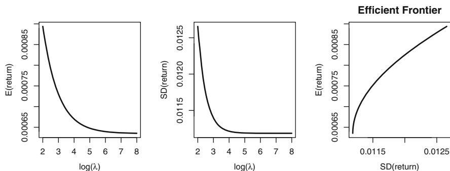
Fig. 16.8. The expected portfolio return versus \log(\lambda) (left), the standard deviation of the return versus \log(\lambda) (center) and the efficient frontier (right).
