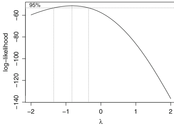
Fig. 11.7. Profile likelihood for the Box-Cox model applied to the simulated data.
