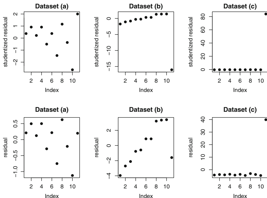
Fig. 10.3. Top row: Externally studentized residuals for the data sets in Fig. 10.1; data set (a) is the data set in panel (a) of Fig. 10.1, and so forth. Case #11 is an outlier in data sets (b) and (c) but not in data set (a). Bottom row: Raw residuals for the same three data sets as in the top row. For data set (b), the raw residual does not reveal that case #11 is outlying.
