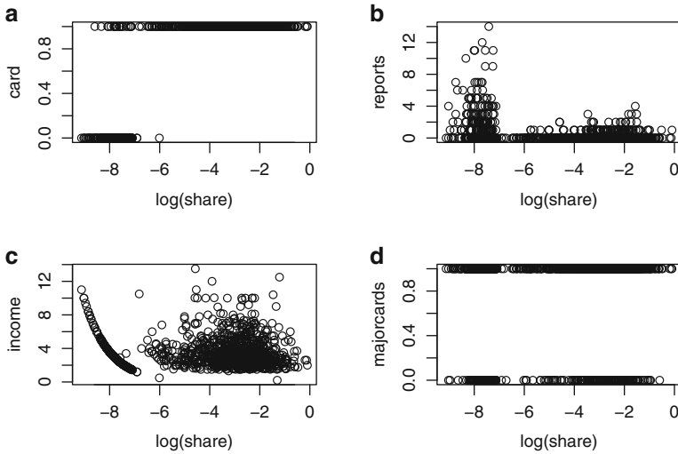
Fig. 11.11. Plots of \log(\text{share}) versus other variables.
