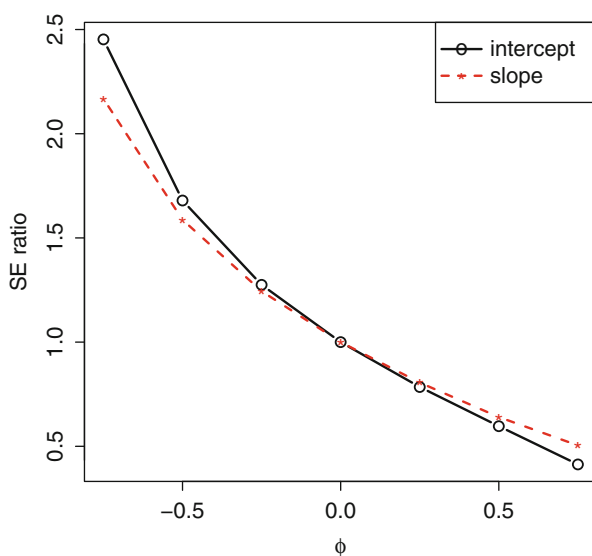
Fig. 13.8. Factor by which the standard error is changed when \phi deviates from 0 for intercept (solid) and slope (dashed).
