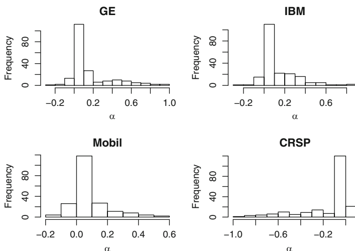
Fig. 7.9. Histograms of 200 bootstrapped values of \hat{\alpha} for each of the returns series in the CRSPday data set.
