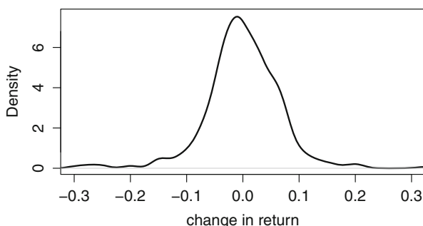
Fig. 5.9. Kernel estimate of the probability density of diffrrf , the changes in the risk-free returns.
