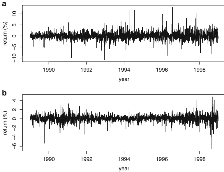
Fig. 14.11. Daily returns (in percentage) for (a) IBM stock and (b) the CRSP value-weighted index, including dividends.
