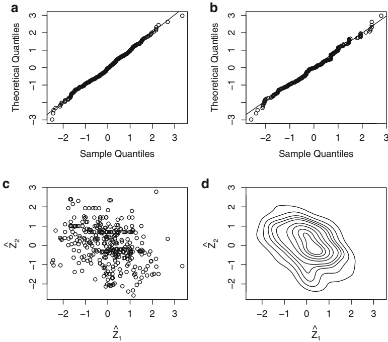
Fig. 8.8. Pipeline data. Normal quantile plots (a) and (b), a scatterplot (c) and KDE density contours for the normal-transformed flows.
