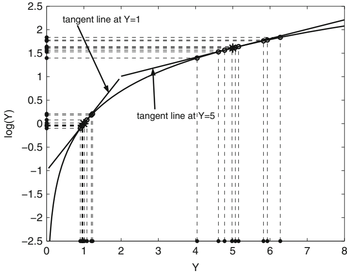
Fig. 4.24. A variance-stabilizing transformation.
