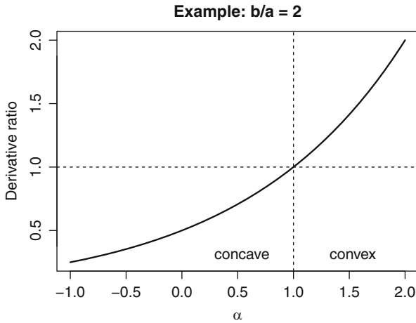
Fig. 4.25. Derivative ratio for Box-Cox transformations.
