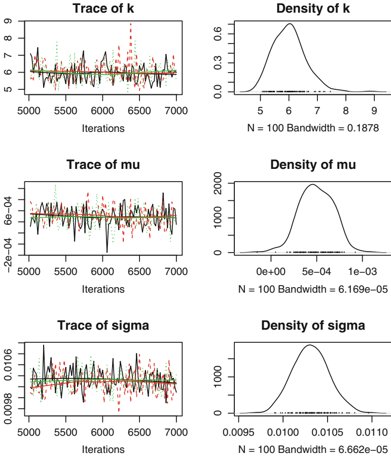
Fig. 20.4. Trace plots and kernel density estimates in Example 20.9.
