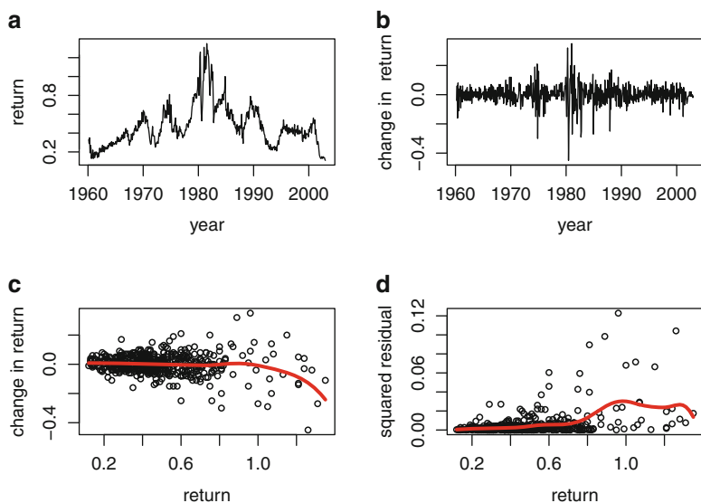
Fig. 21.1. Risk-free monthly returns. The returns are 1/12th the yearly rate. (a) Time series plot of the returns. (b) Time series plot of the changes in the returns. (c) Plot of changes in returns against lagged returns with a local linear estimate of the drift. (d) Plot of squared residuals against lagged returns with a local linear estimate of the squared diffusion coefficient.
