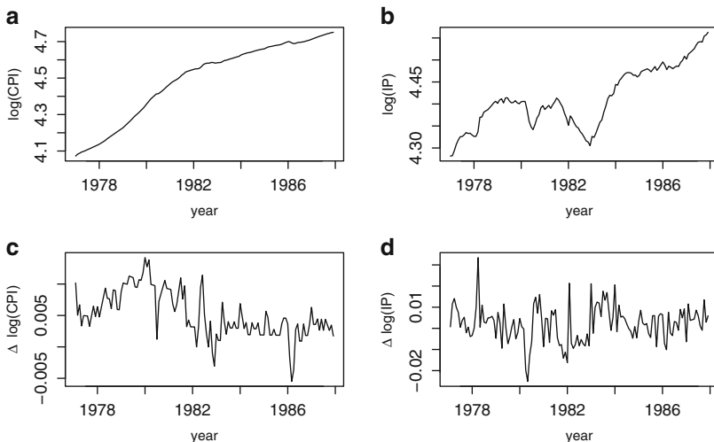
Fig. 13.11. (a) Time series plot of \log(\text{CPI}) (b) Time series plot of \log(\text{IP}) (c) Time series plot of changes in \log(\text{CPI}) (d) Time series plot of changes in \log(\text{IP}) .
