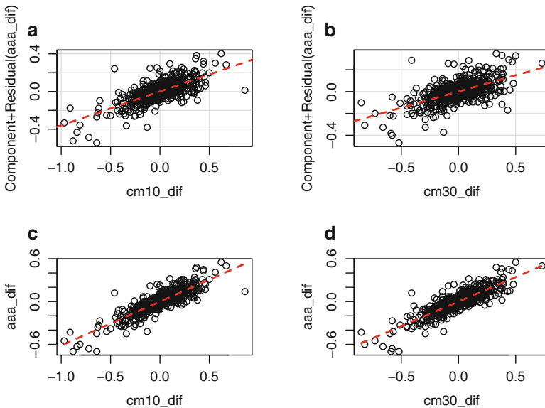
Fig. 9.7. Partial residual plots for the weekly interest rates [panels (a) and (b)] and scatterplots of the predictors and the response [panels (c) and (d)].
