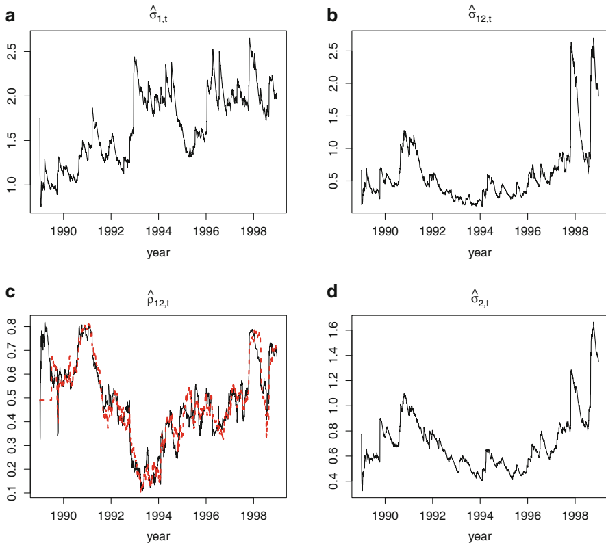
Fig. 14.14. A fitted EWMA model with \lambda = 0.985 . The red line in (c) is the sample correlation estimate over the previous six months for comparison.
