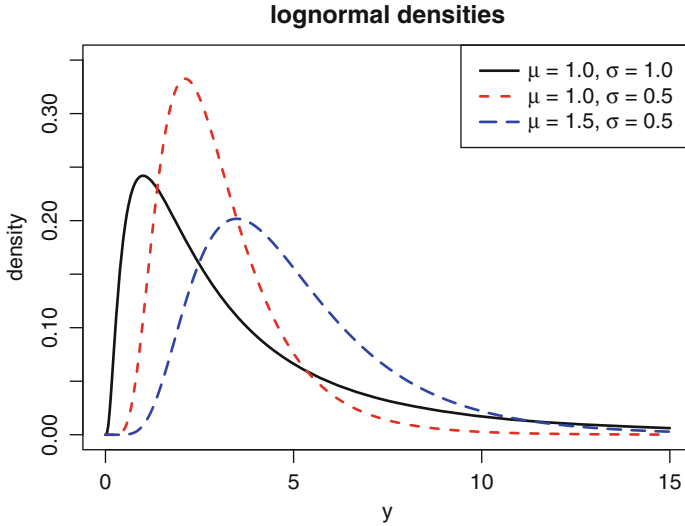
Fig. A.1. Examples of lognormal probability densities. Here \mu and \sigma are the log-mean and log-standard deviation, that is, the mean and standard deviation of the logarithm of the lognormal random variable.
