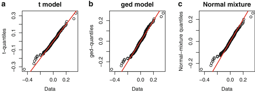
Fig. 5.10. (a) QQ plot of diffrrf versus the quantiles of a t_{\nu}^{\text{std}}(\mu, s^2) distribution with \mu , s^2 , and \nu estimated by maximum likelihood. A 45^\circ line through the origin has been added for reference. (b) A similar plot for the generalized error distribution. (c) A similar plot for a normal mixture model.
