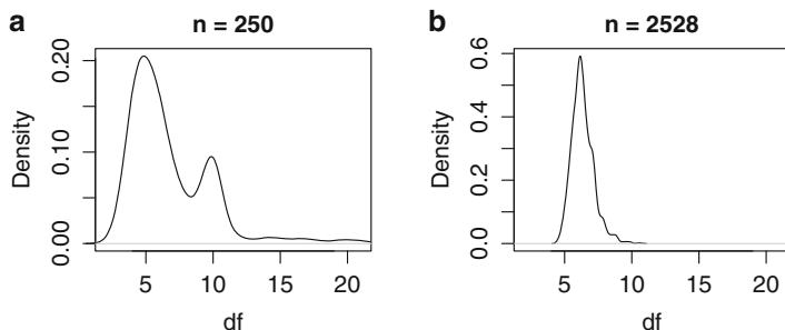
Fig. 6.1. Kernel density estimates of 1,000 bootstrap estimates of df using (a) the first 250 daily GE returns and (b) all 2,528 GE returns. The default bandwidth was used in R's density function to create the estimates.
