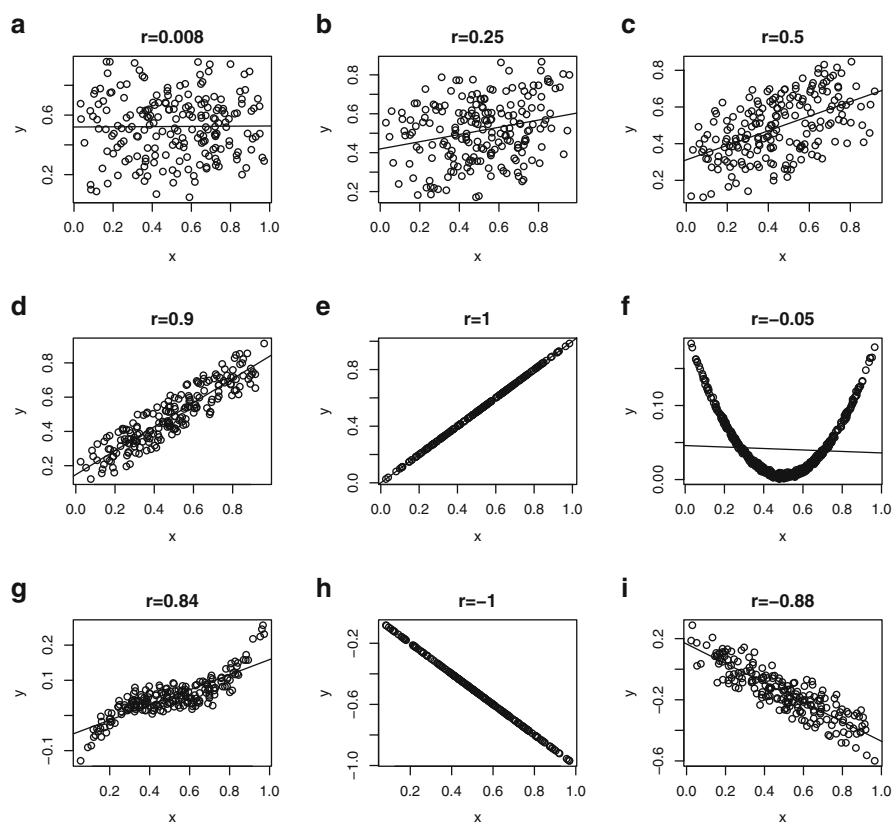
Fig. A.4. Sample correlation coefficients for nine random samples. Each plot also contains the linear regression line of y on x .
