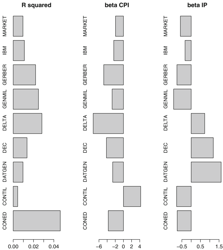
Fig. 18.6. R^2 and slopes of regressions of stock returns on CPI residuals and IP residuals.
