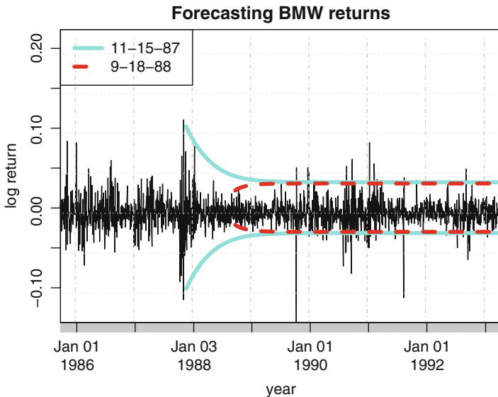
Fig. 14.10. Prediction limits for forecasting daily BMW stock log returns from two different time origins.
