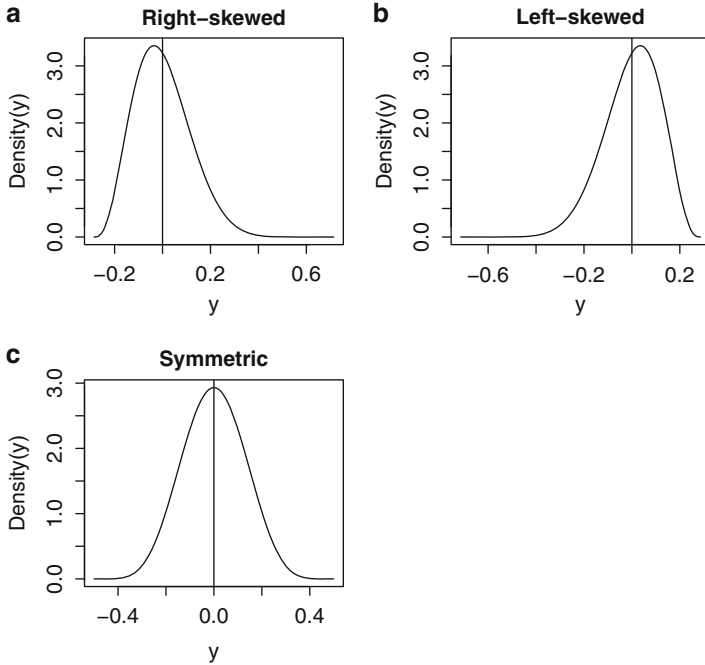
Fig. 5.1. Skewed and symmetric densities. In each case, the mean is zero and is indicated by a vertical line. The distributions in panels (a)–(c) are \text{beta}(4,10) , \text{beta}(10,4) , and \text{beta}(7,7) , respectively. The R function dbeta() was used to calculate these densities.
