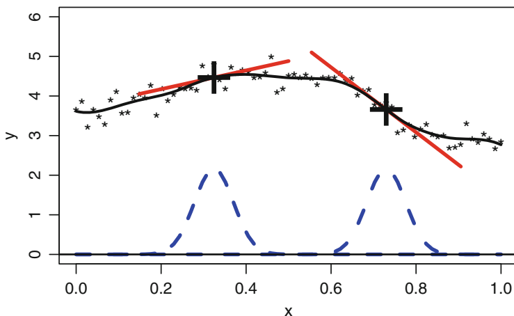
Fig. 21.2. Local linear fit (solid curve) to 75 data points (asterisks) with bandwidth chosen by the direct plug-in method. The regression function \mu is estimated at each of the 75 points and the estimates are connected to create the solid curve. Estimation at x_{25} = 0.32 and x_{55} = 0.72 is illustrated by the kernels (dashed curves), the linear fits (solid lines), and the fitted points (large +).
