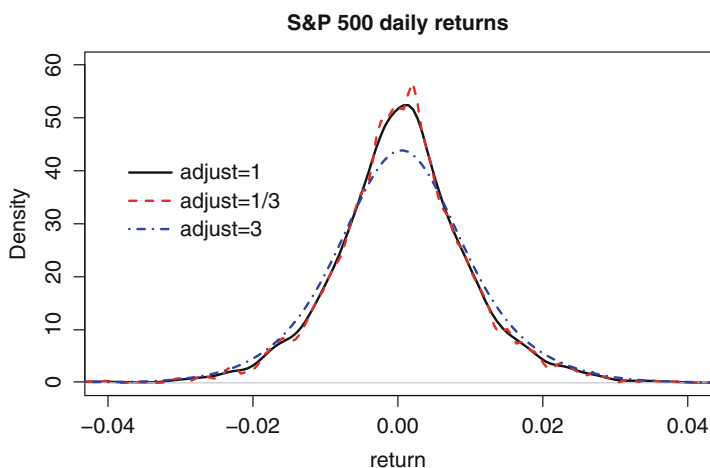
Fig. 4.6. Kernel density estimates of the daily log returns on the S&P 500 index using three bandwidths. Each bandwidth is the default bandwidth times adjust and adjust is 1/3 , 1 , and 3 . This data set is the SP500 series in the Ecdat package in R. The KDE is plotted only for a limited range of returns to show detail in the middle of the distribution.
