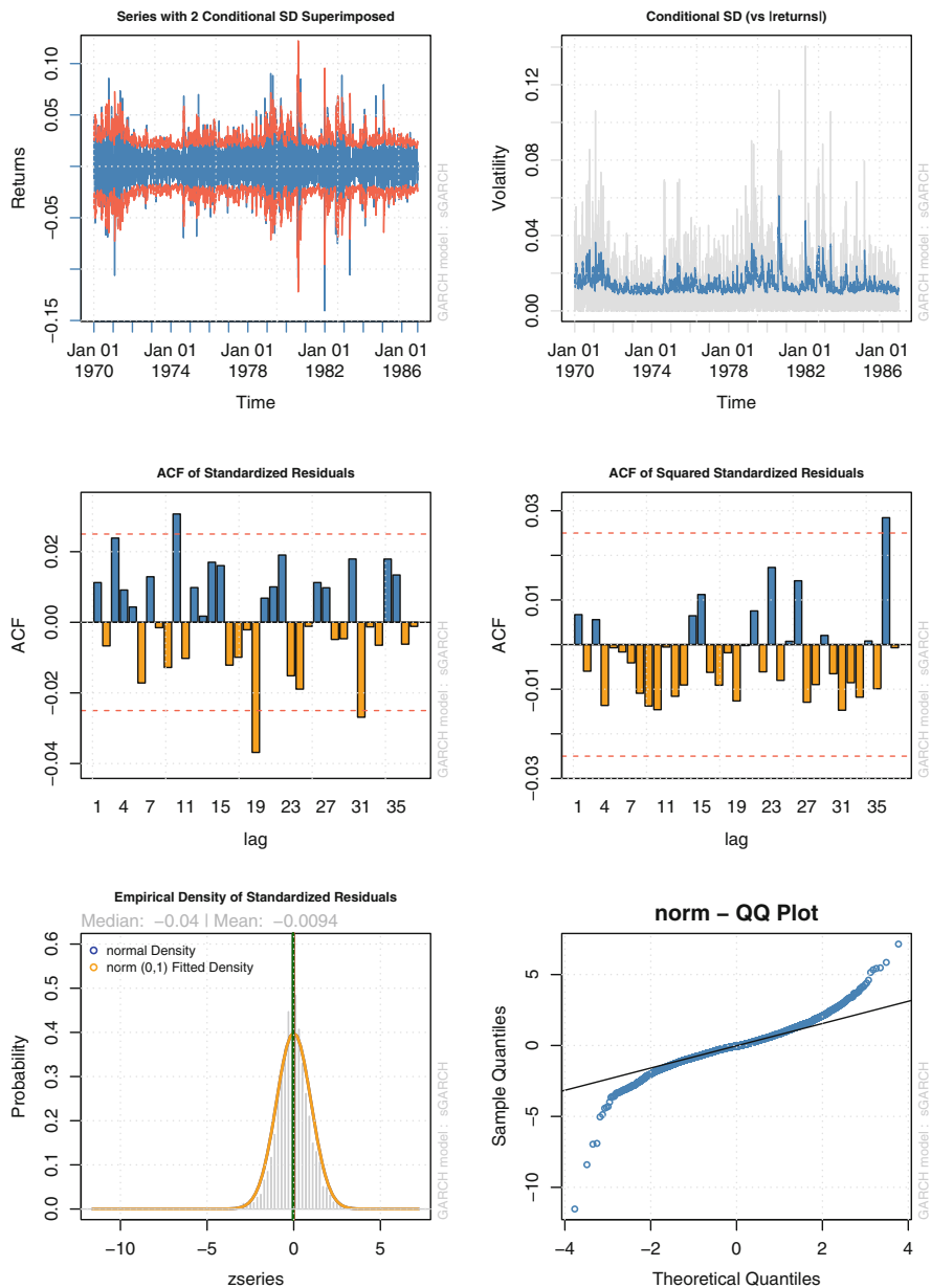
Fig. 14.4. The daily BMW stock log return series Y_t , with two estimated conditional standard deviations superimposed; the estimated conditional standard deviation \hat{\sigma}_t series (vs. the absolute value of the log return series |Y_t| ); the sample ACF of the standardized residuals \hat{\epsilon}_t and the squared standardized residuals \hat{\epsilon}_t^2 ; empirical density estimates of the standardized residuals \hat{\epsilon}_t ; and a normal quantile plot of the standardized residuals \hat{\epsilon}_t .
