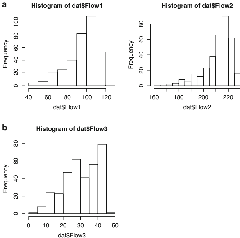
Fig. 4.20. Histograms of daily flows in three pipelines.
